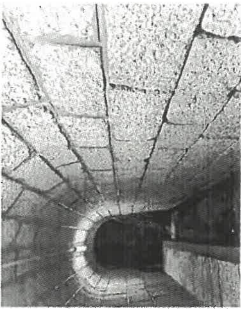
Figure 2. Water catchment object – Mošćanica river source
